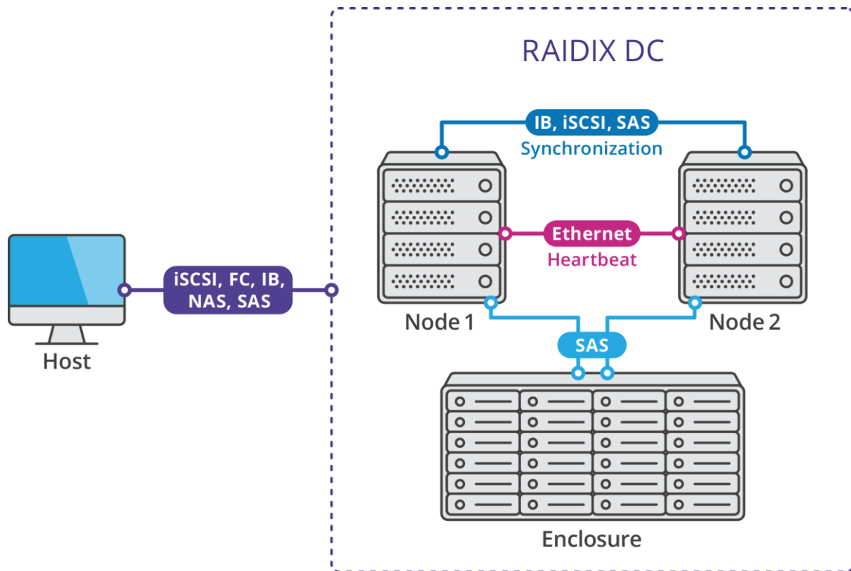
Figure 2. RAIDIX 5.0.1 Dual-controller mode
